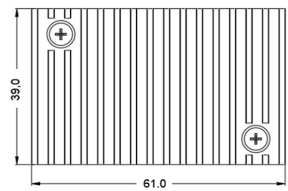
Standard+Heatsink 61.0x39.0x27.7mm
