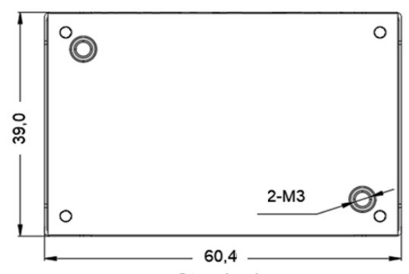
Standard 60.4x39.0x12.7mm
